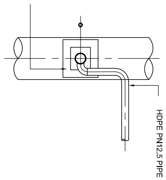
PLAN (TYPE '3')
