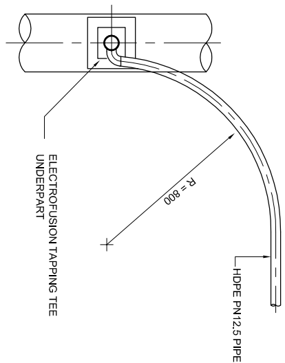
PLAN (TYPE '2')
